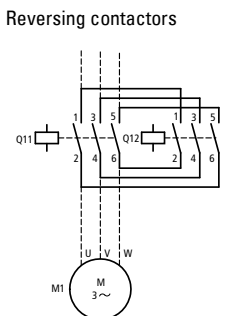
DIULM7/21 to DIULM65/11 with mechanical interlock
